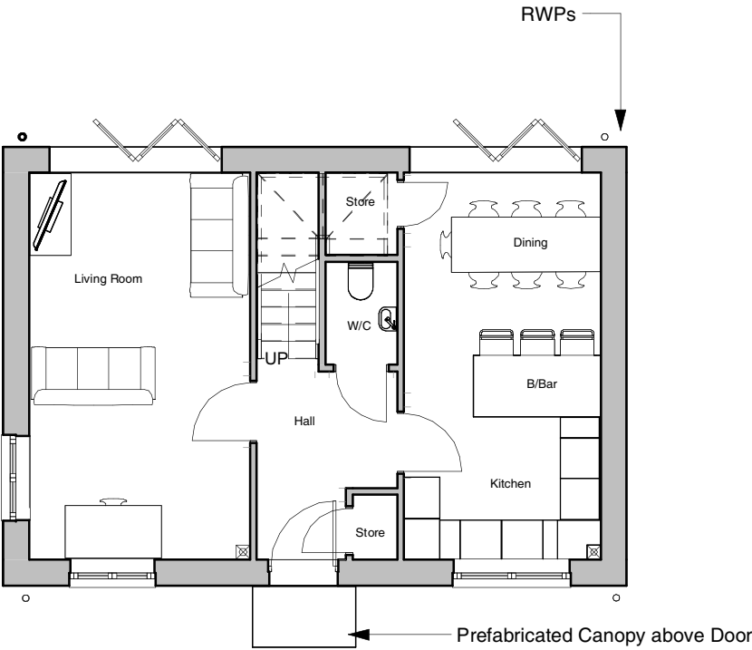
1 Housetype D Ground Floor 1 : 100
