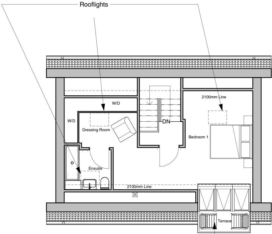
3 Housetype D Second Floor 1 : 100
