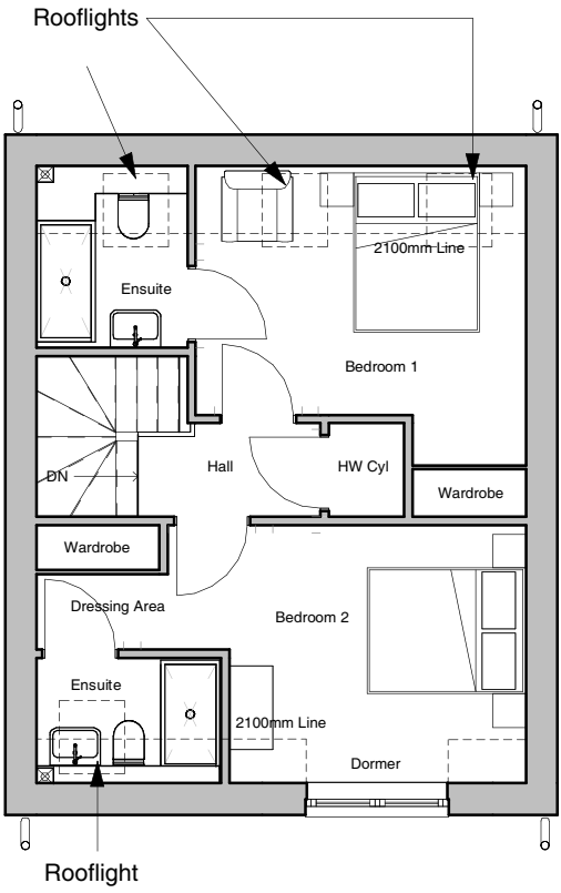
3 Housetype B Second Floor 1 : 100
